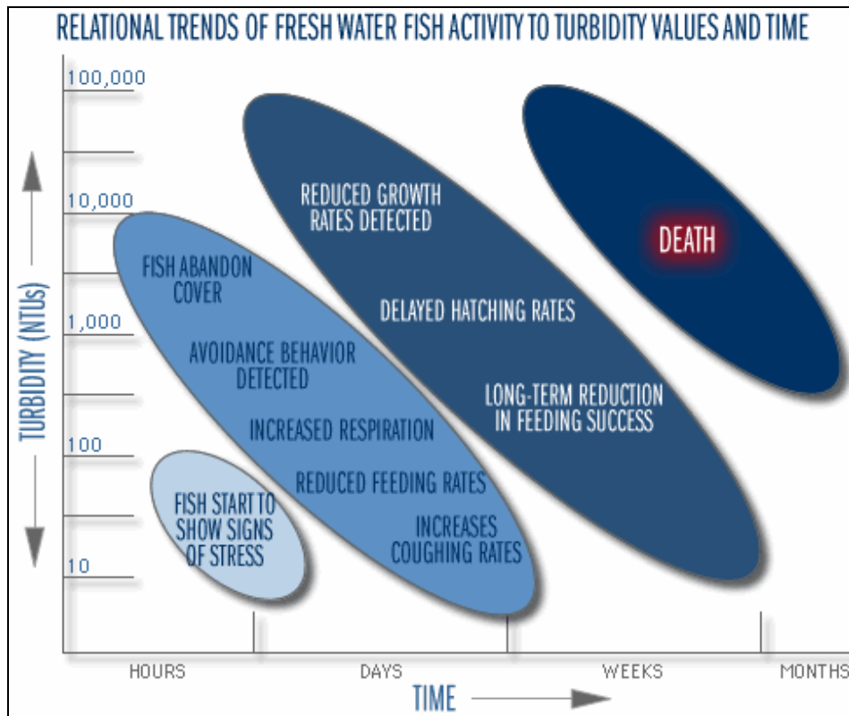
Fig. 1 The relational trends between freshwater fish activity and turbidity values over time
